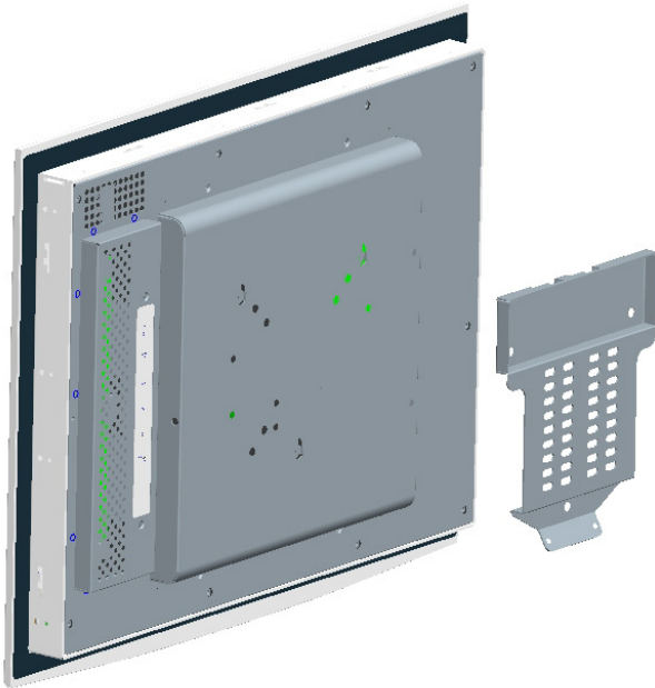
Figure 2.1: Wallmounting
