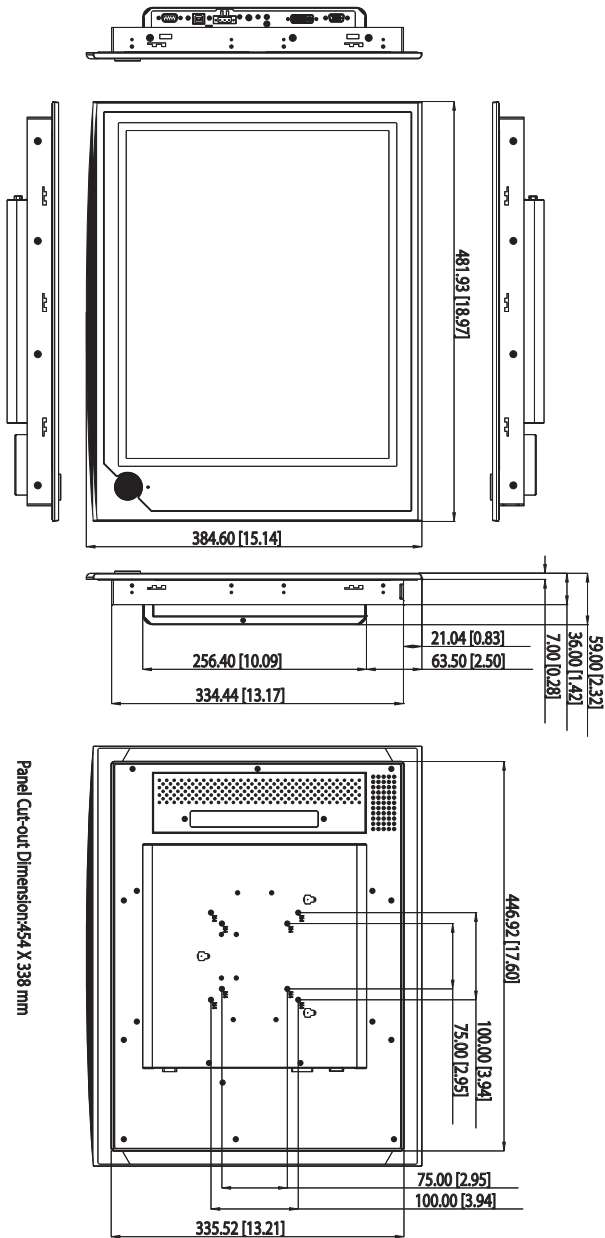
Figure 1.1: FPM-5191G Dimensions
